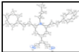
Fig. 1. The structure of the title compound, with displacement ellipsoids drawn at the 30% probability level for non-H atoms.
